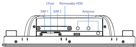
Rear I/O
