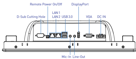
Rear I/O
