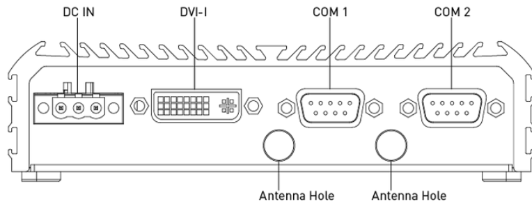
Rear Panel
