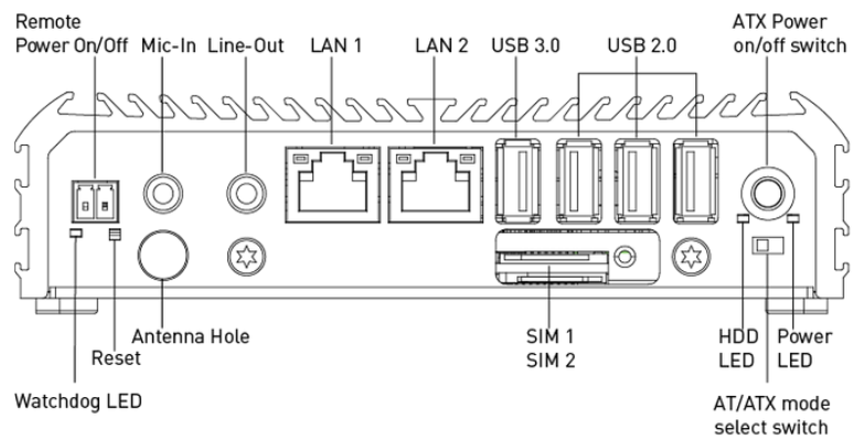
Front Panel
