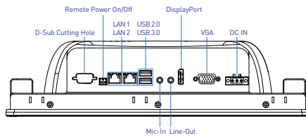
Rear I/O
