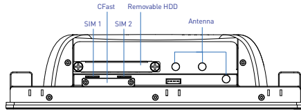
Rear I/O
