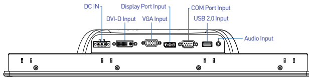
Rear I/O
