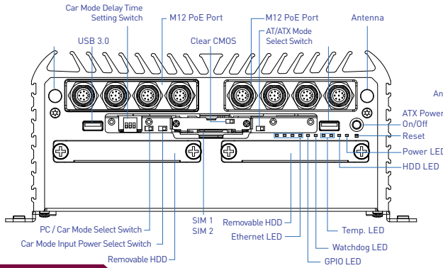
Front Panel
