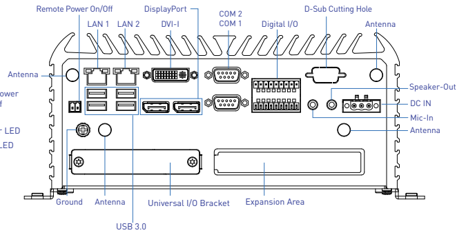
Rear Panel
