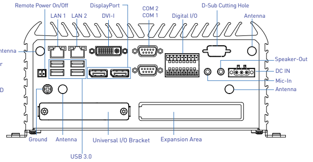
Rear Panel
