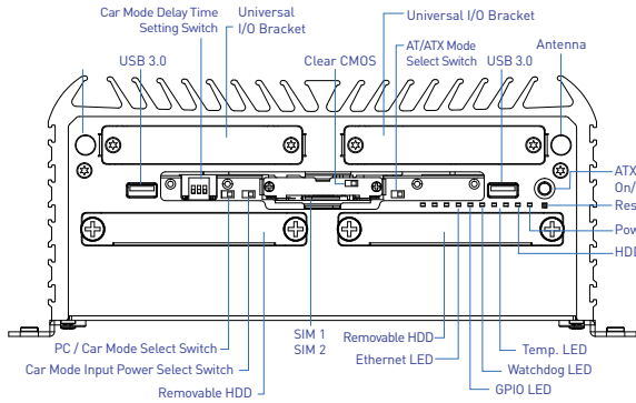
Front Panel
