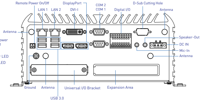
Rear Panel
