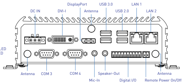
Rear Panel
