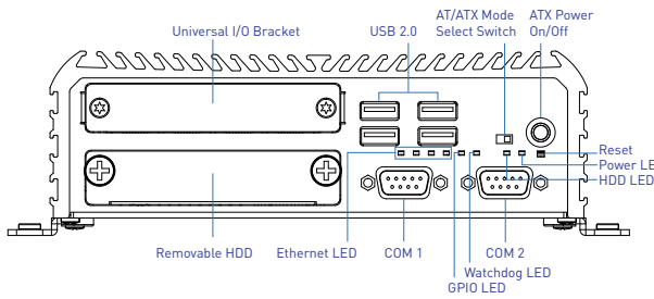
Front Panel
