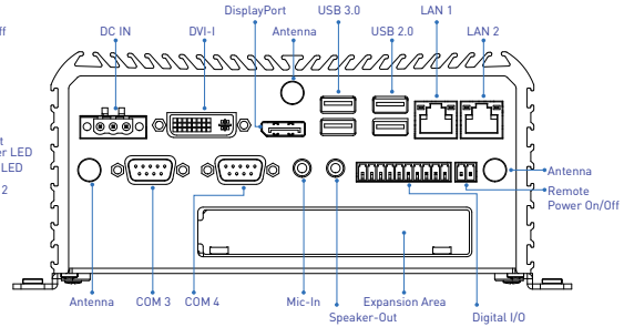
Rear Panel
