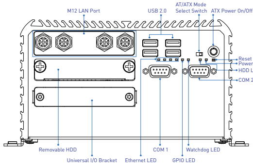
Front Panel
