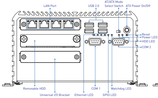
Front Panel
