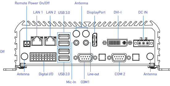
Rear Panel
