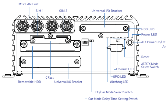
Front Panel
