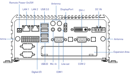
Rear Panel
