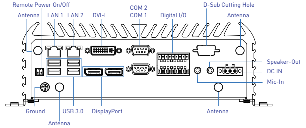
Rear Panel
