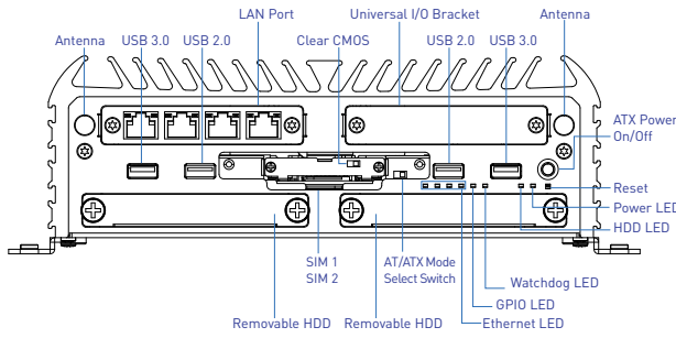
Front Panel
