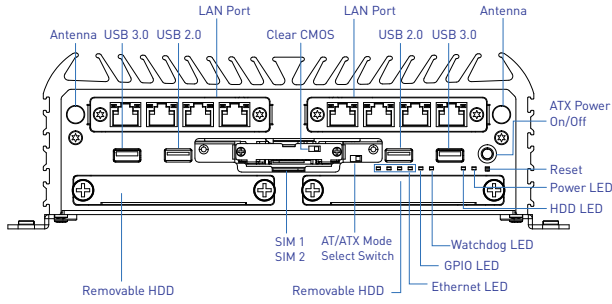
Front Panel
