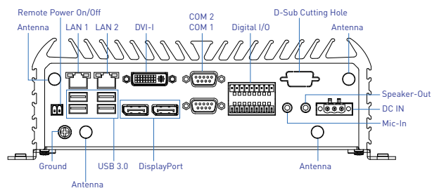
Rear Panel
