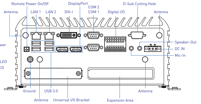
Rear Panel
