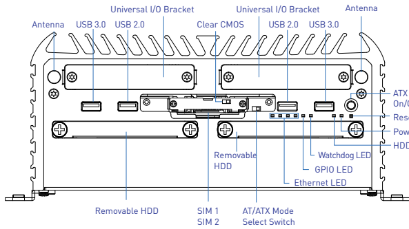
Front Panel
