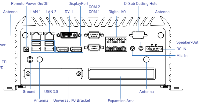
Rear Panel
