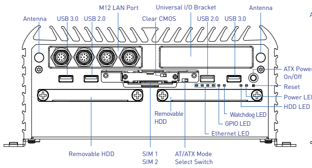
Front Panel
