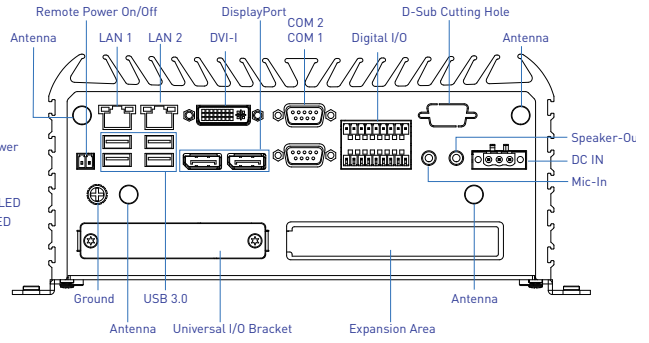
Rear Panel
