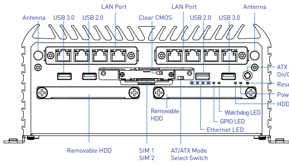
Front Panel
