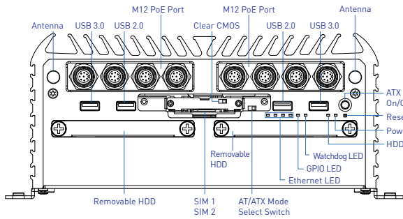
Front Panel
