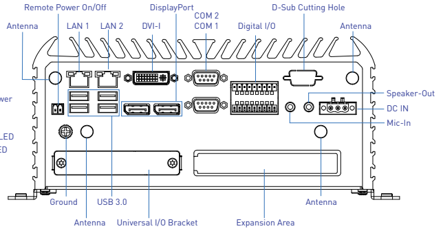
Rear Panel
