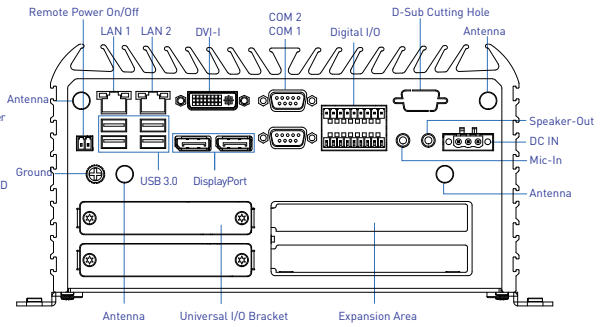
Rear Panel
