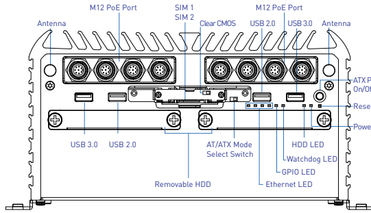
Front Panel
