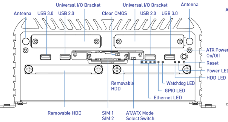
Front Panel
