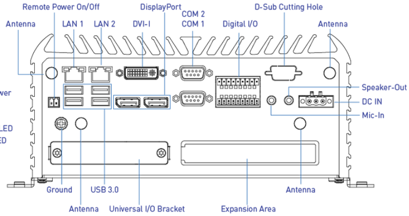
Rear Panel
