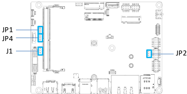
JP1:Clear CMOS, 1*3P, Pitch, 2.00mm
