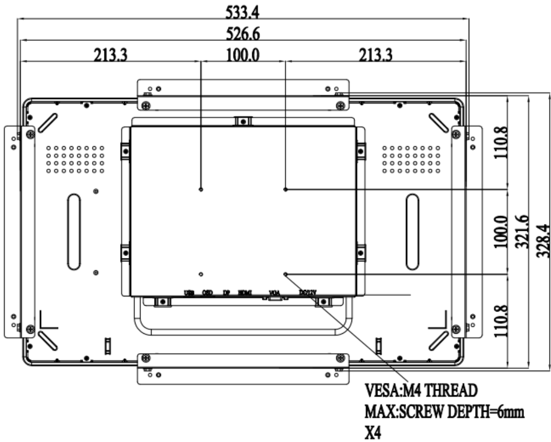
VESA installation holes
