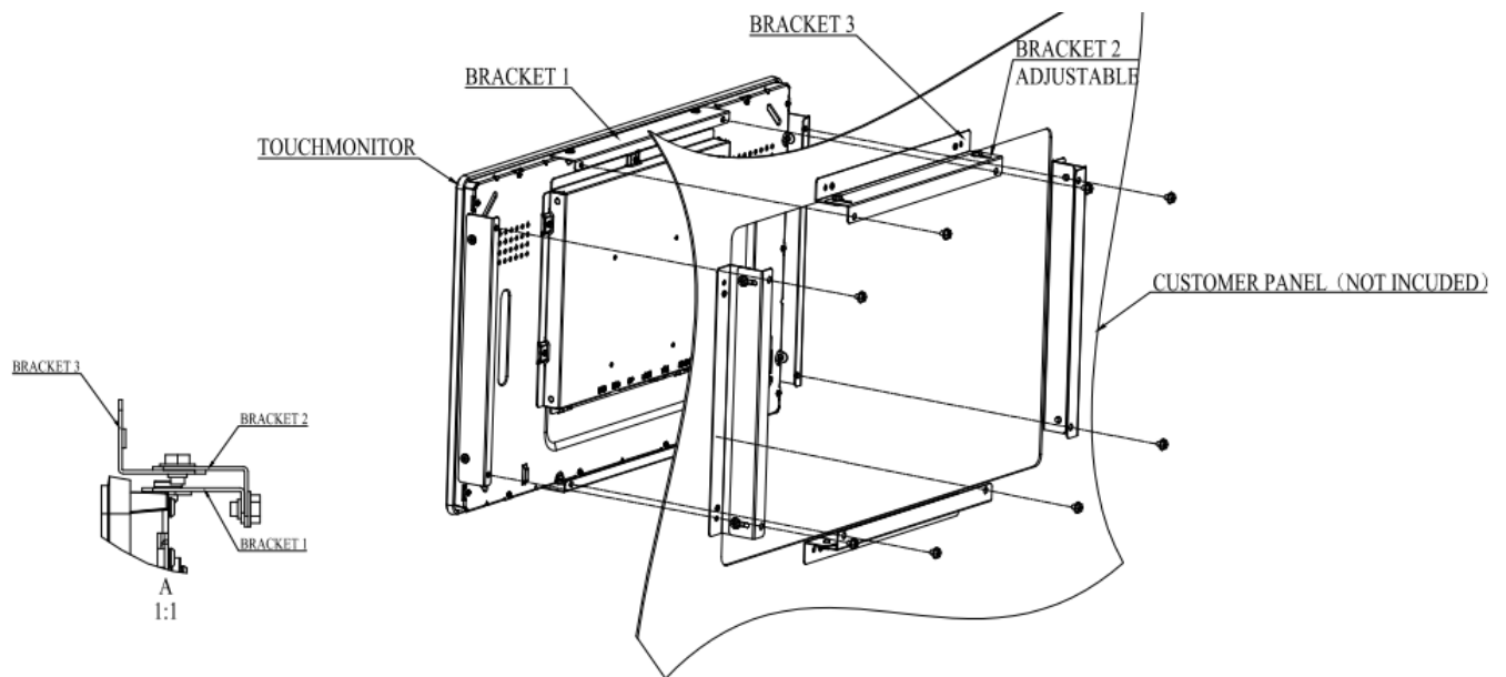
Rear mounting
