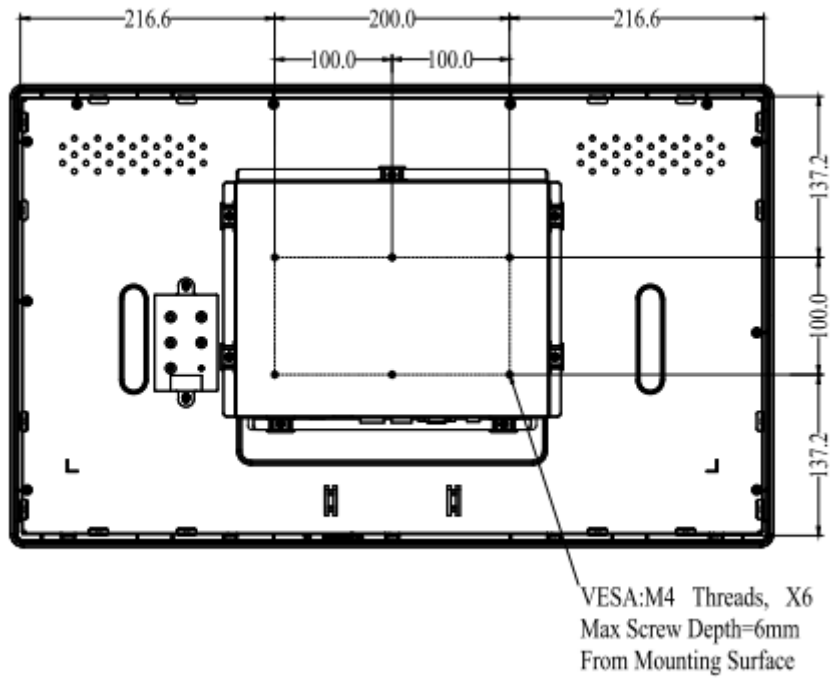
VESA installation holes
